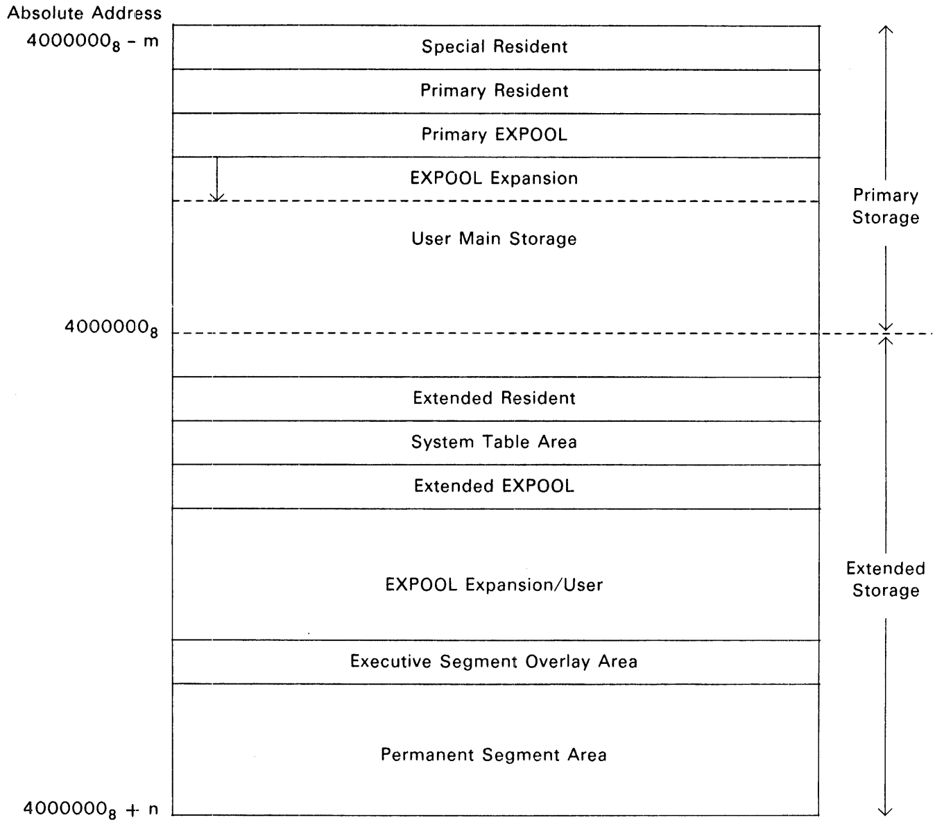
Figure 12-2. 1110, 1100/40 Main Storage
