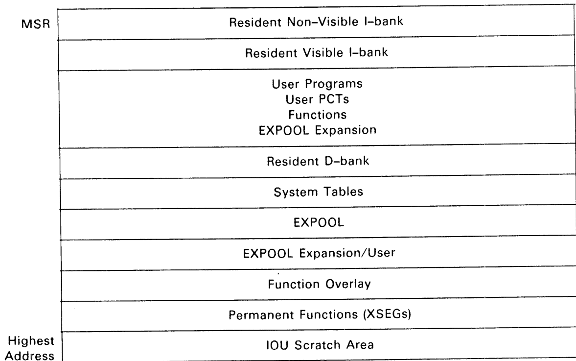
Figure 12-3. 1100/80 Main Storage
